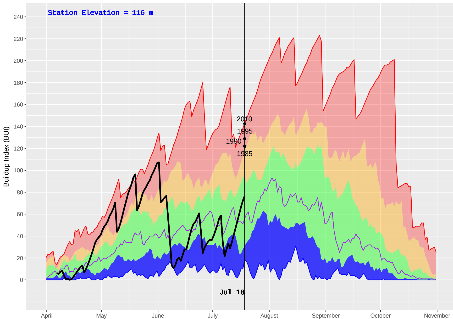
SCAR CREEK (82) : Historical (1982–2016) and Current (2018) Daily Buildup Index (BUI)
